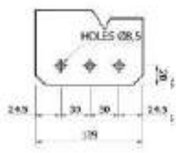
DETAIL OF DRILLING INTERNAL BAR
