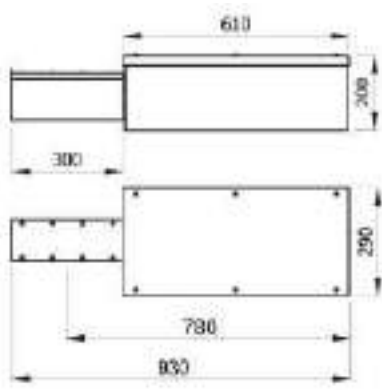
DETAIL OF DRILLING INTERNAL BAR
